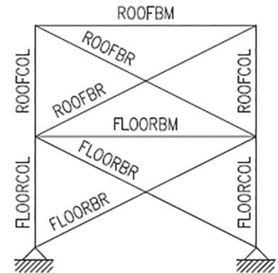
Fig. 3-5. Braced frame member labels.
