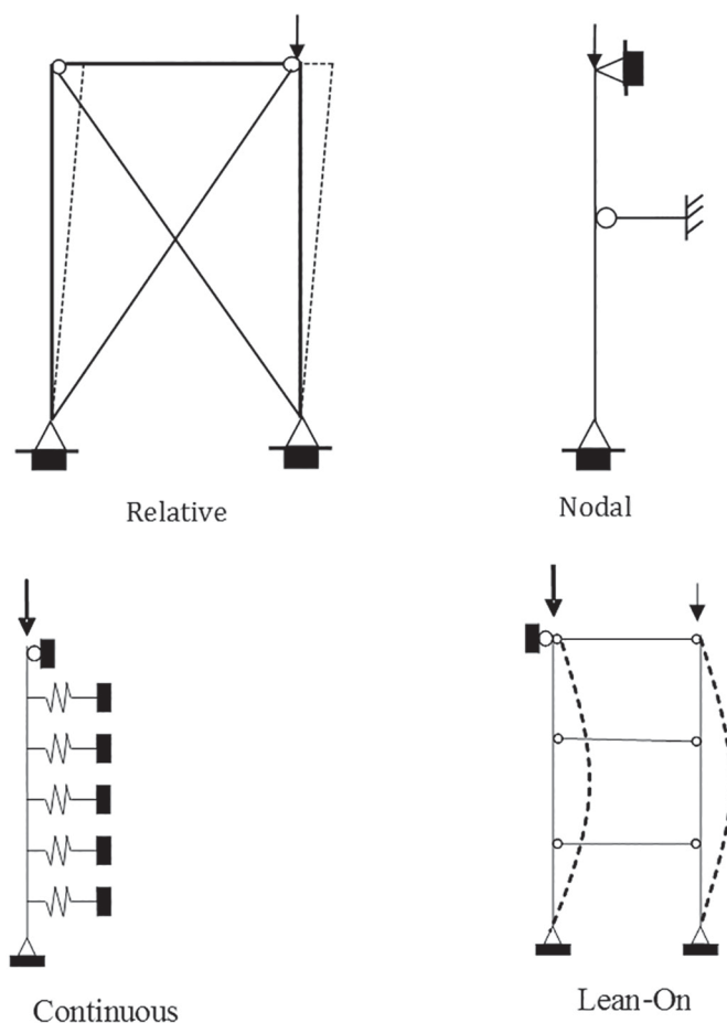
Fig. E-1. Types of column bracing.
