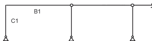
Fig. 4-6. North-south moment frame.
