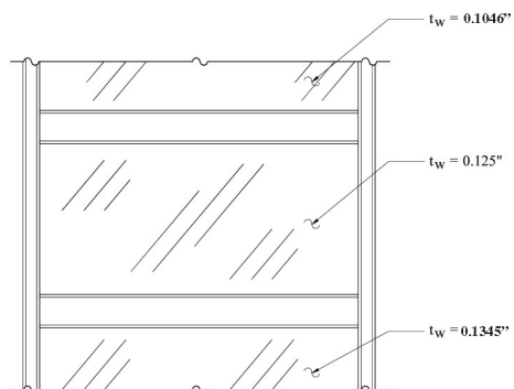
Fig. 6–5. SPSW panel without opening.
