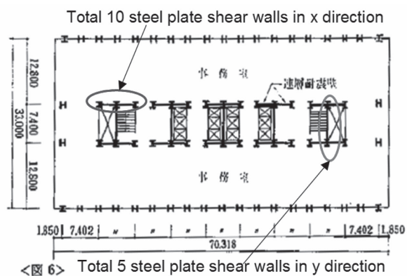
Fig. 1-6. Plan layout of SPW for Nippon Steel Building (Yokoyama et al., 1978).
