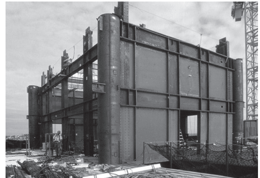
Fig. 1–20. Core walls with composite concrete infill steel pipe columns (Seilie and Hooper, 2005).
