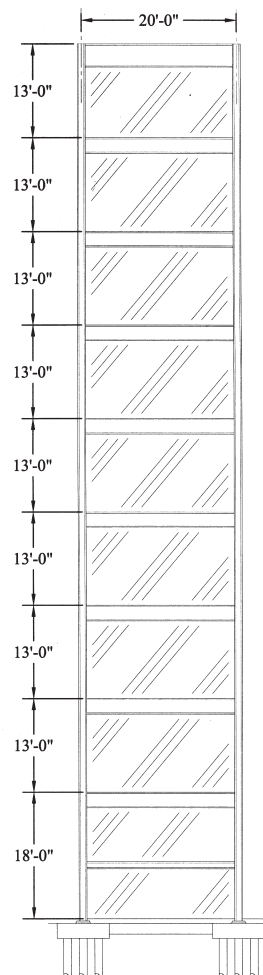
Fig. 4-2. SPW elevation.
