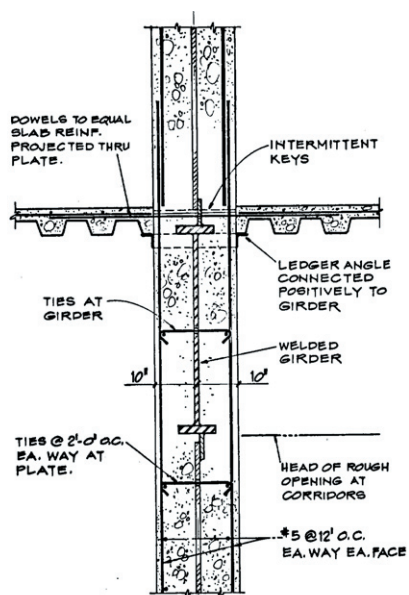
Fig. 1-12. H.C. Moffit Hospital Addition, typical steel shear wall, and example cross-section (Dean et al., 1977; Wosser and Poland, 2003).
