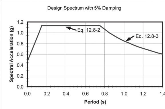
Fig. 5-3. Generalized site response spectrum.
