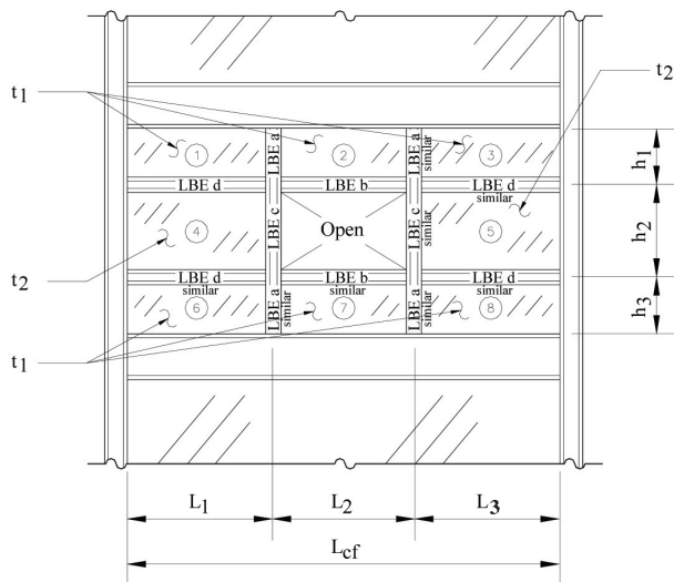
Fig. 6-2. SPSW with opening.
