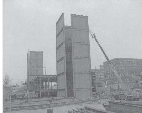
Fig. 1–31. Core wall at middle of ING building (courtesy of Louis Crepeau and Jean-Benoit Ducharme, Groupe Teknika, Montreal, Canada).
