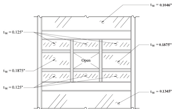
Fig. 6–6. SPSW panel with opening.
