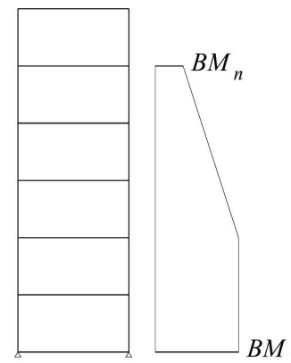
Fig. 3–24. Schematic of ICD overturning moment.
