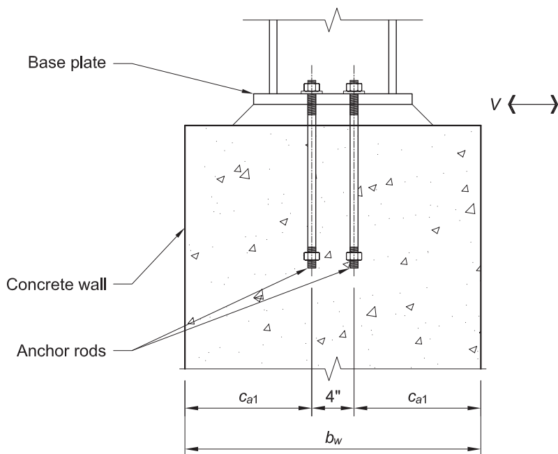
Fig. 4-24. Base connection section for configuration used in Example 4.7-4.
