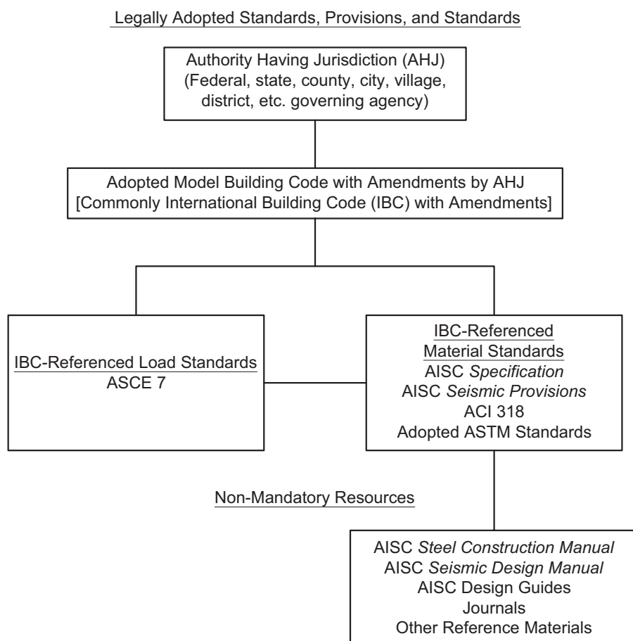
Fig. I-2. Documents relevant to column base and anchorage design.
