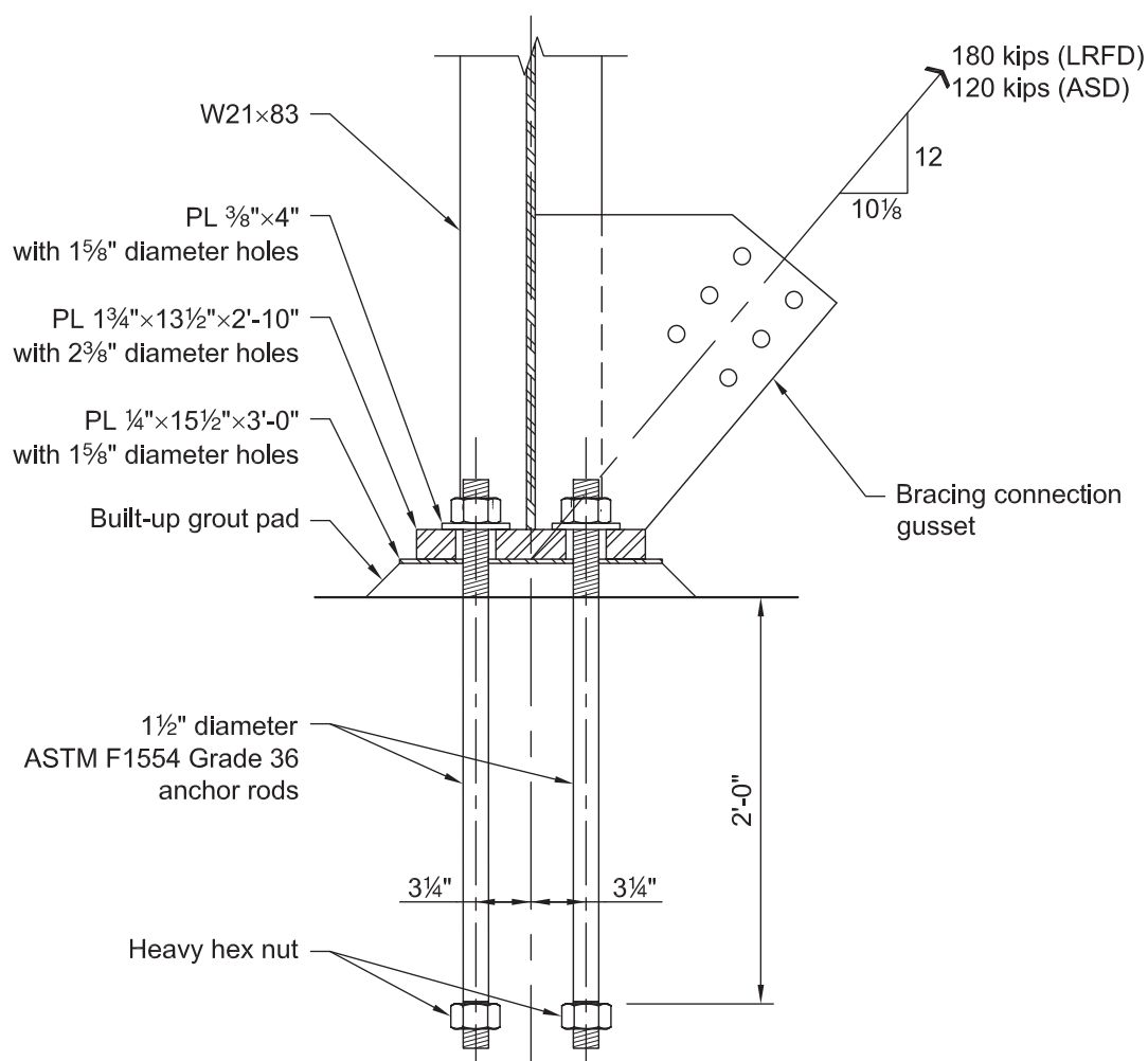
Fig. 4-28. Base connection as detailed in Example 4.7-7.
