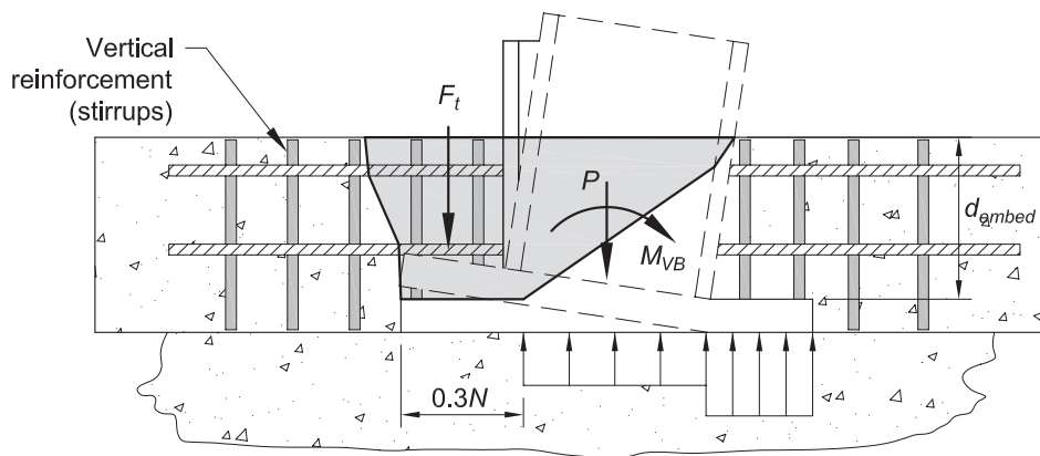
Fig. 5-7. Breakout force of concrete above the tension side of the connection.
