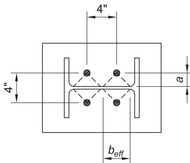
Fig. 4-22. Rod load distribution.
